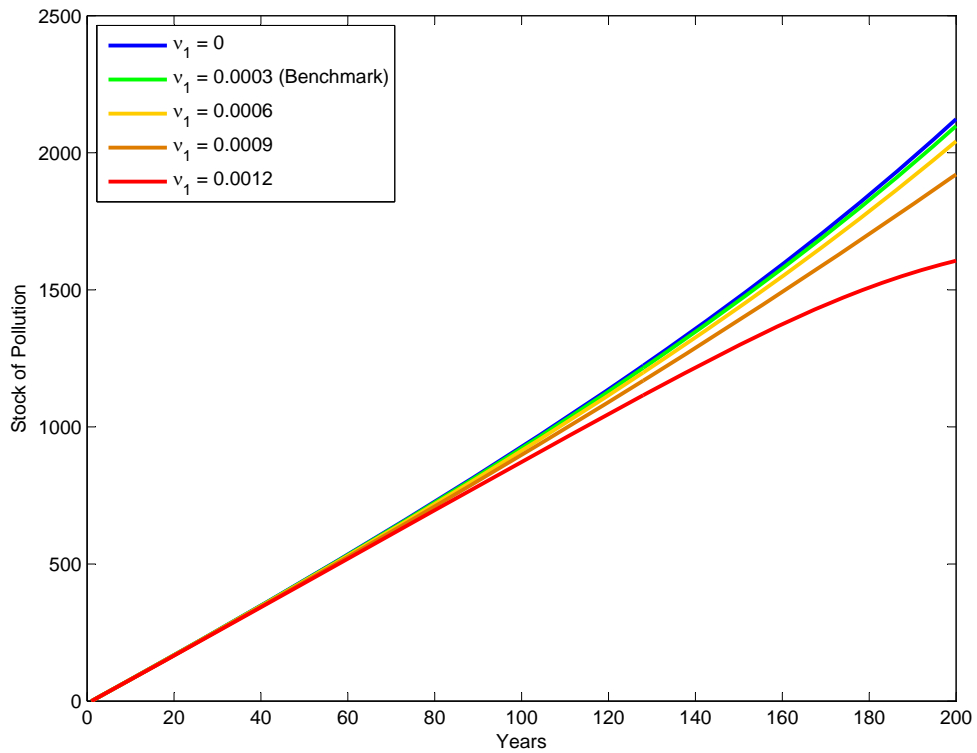
Figure 7. Pollution for Different Values of \nu_1
